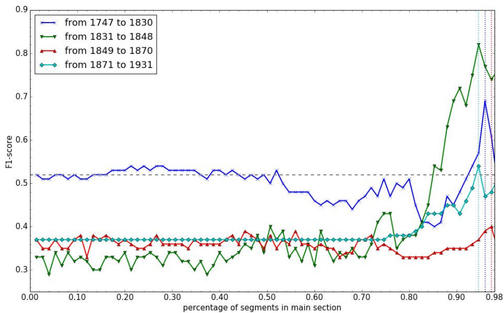
Figure 2: Classification F1-score for different partitionings into main and final section. Each line denotes novels from a different time period. The dashed line represents the random baseline for the time period starting from 1871. Random baselines for the other periods yield slightly worse results and are omitted. The dotted lines show where the maximum F1-score is reached for the respective time periods.
